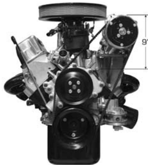
289-351W Driver Side Power Steering Bracket (add on kit) 131108
