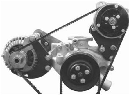
383-440 Mopar Compressor and Alt Brt 161002
